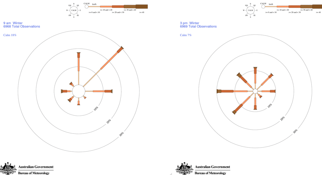
Figure 6. Wind roses depicting Perth wind conditions during Winter at 9am (left) and 3pm (right).
