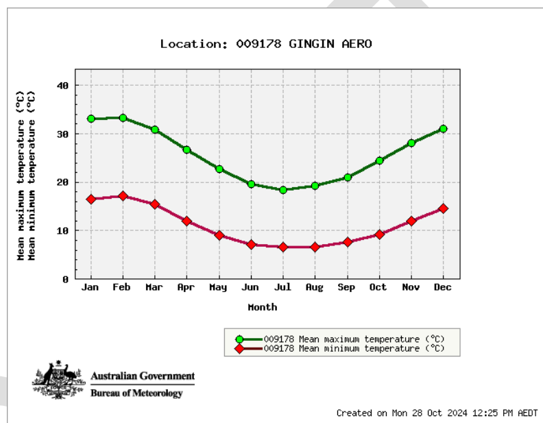
Figure 3. Mean maximum and minimum monthly temperatures recorded at Gingin weather station, approximately 20km from Yanchep Lagoon.
