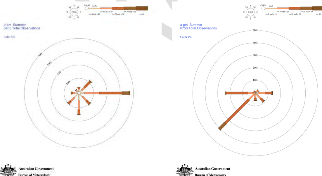
Figure 5. Wind roses depicting Perth wind conditions during Summer at 9am (left) and 3pm (right).
