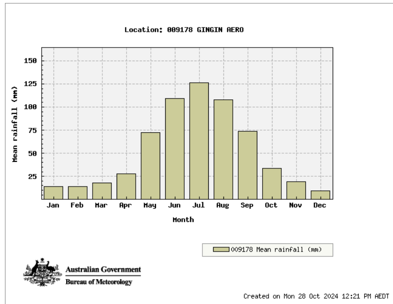
Figure 4. Mean rainfall recorded at Gingin weather station, approximately 20km from Yanchep Lagoon.
